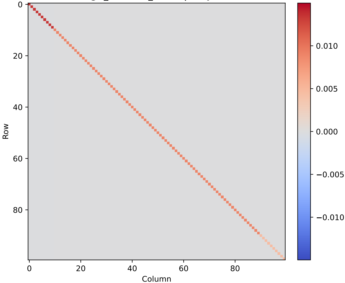
gd_random_small | step 5
